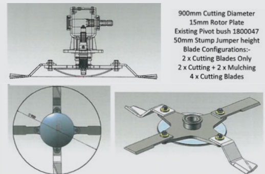
Batwing Rotor design (4 blade)
